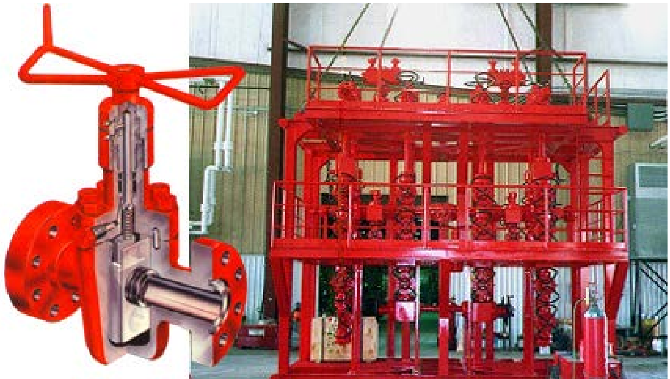
Choke and Kill Manifold 4-1/16" – 15,000 PSI WP
